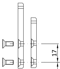
viti trilobate | lobed screws M4x8* - CV1243I
