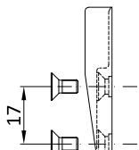
viti trilobate | lobed screws M4x8* - CV1243I
