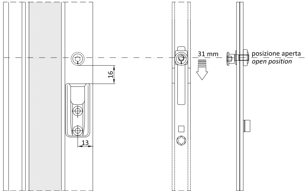
Riscontri anti falsa manovra Mishandling device strike
