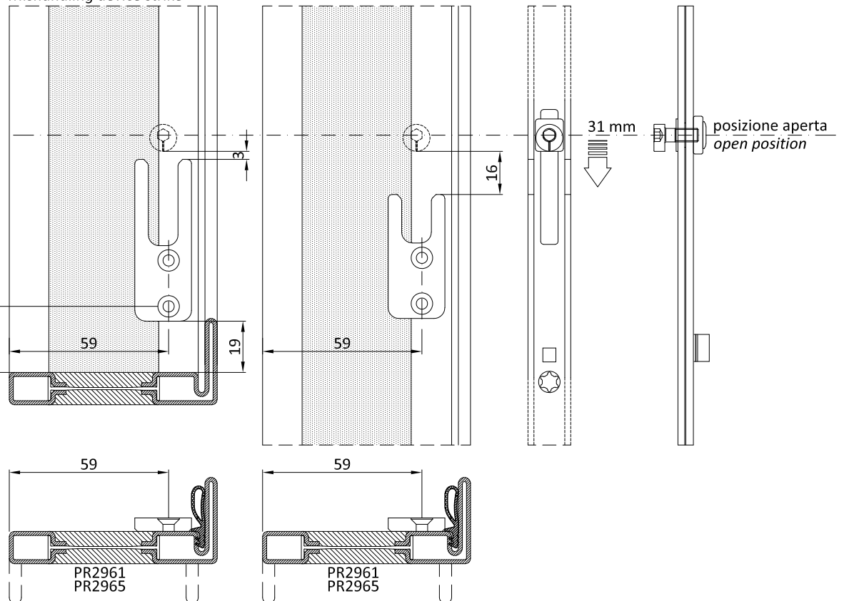
Riscontri anti falsa manovra Mishandling device strike
